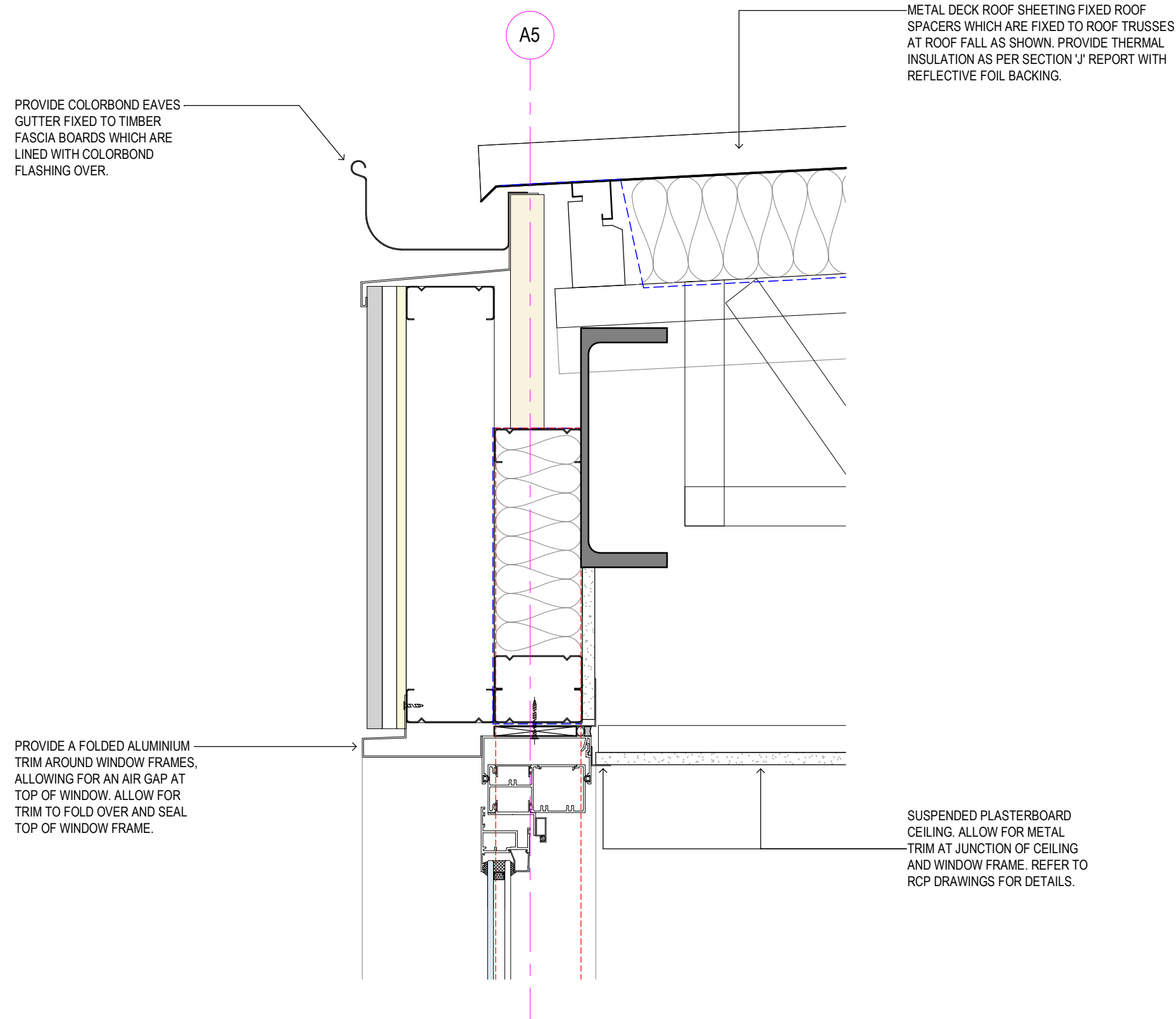
22 DETAIL 22 Scale 1:5
