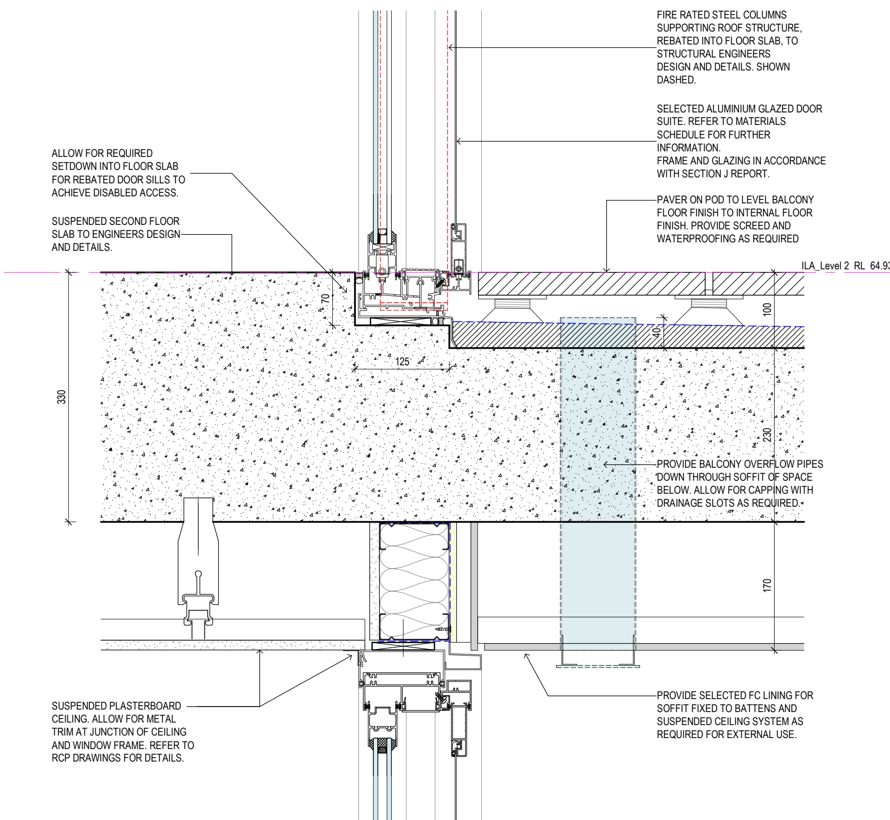
21 DETAIL 21 Scale 1:5
